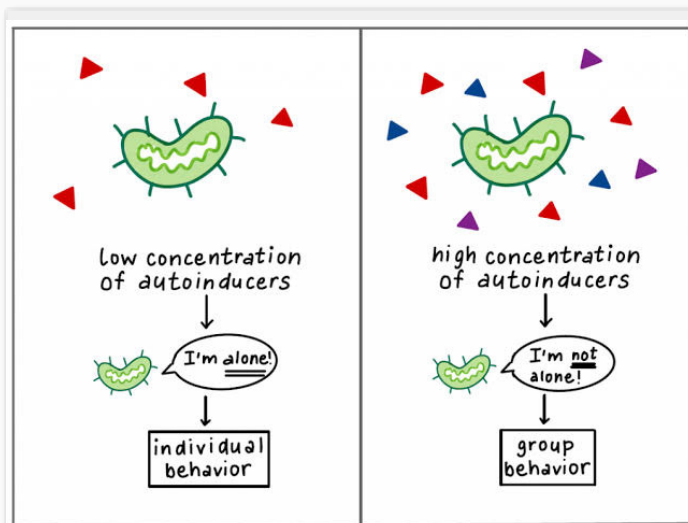
Fig 3. Live Application treatments often suffer from short activation periods, lowering effectiveness and requiring frequent reapplication. This system regulates GM bacteria to oscillate around a set population, enhancing linalool output and media conservation, extending product usability over time. [IISER Kolkata iGEM 2024 Wiki]
