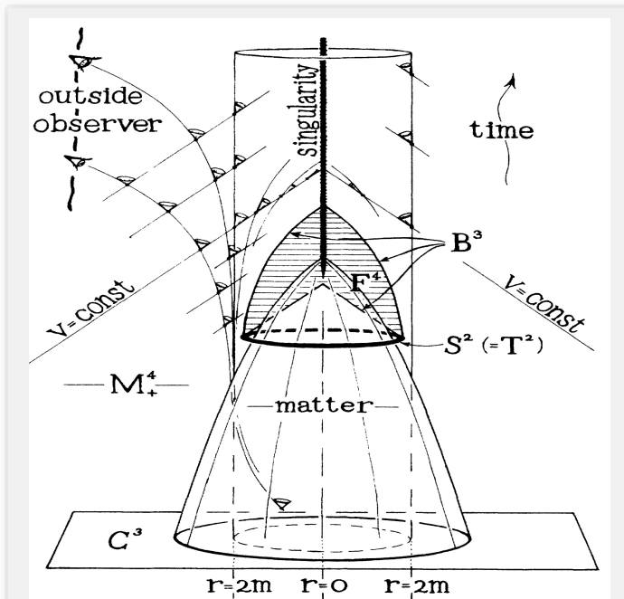
Fig 7. In his 1965 paper, Penrose included this diagram to illustrate how matter undergoes gravitational collapse during the formation of a black hole. Time is represented along the vertical axis, while light rays travel at 45-degree angles, entering the black hole and continuing toward the central singularity. See [9].
