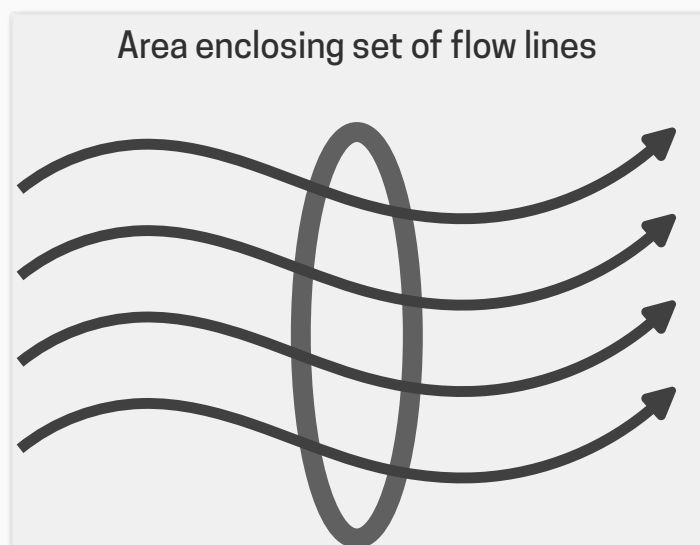
Fig 5. Trajectories of particles governed by Einstein's equations can be thought of as a fluid moving through space. The Raychaudhuri equation describes how the area of the flow depends on various factors.
