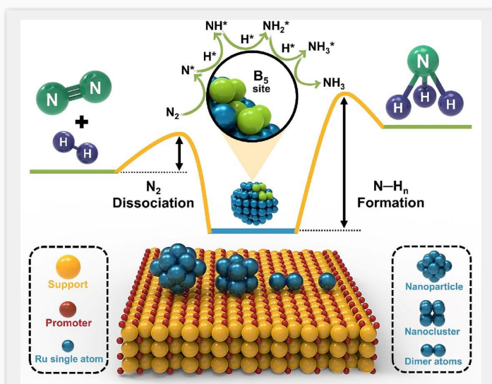
Fig 5. New advancements in ammonia synthesis include the use of single-atom ruthenium (Ru) catalysts, which significantly increase catalytic efficiency by maximising active site exposure and enhancing structural sensitivity. These Ru catalysts enable efficient ammonia production through thermocatalysis, photocatalysis, and electrocatalysis while reducing reaction energy requirements.
