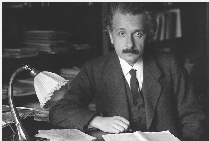
Fig 3. In 1919, Arthur Eddington's team confirmed Einstein's General Theory of Relativity by observing the bending of light from stars near the Sun during a solar eclipse, with observations made in Principe (West Africa) and Sobral (Brazil). This groundbreaking discovery validated Einstein's ideas about gravity and spacetime, propelling him to global fame.
