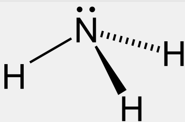
Fig 3. Ammonia ( \text{NH}_3 ) is a simple molecule composed of one nitrogen atom and three hydrogen atoms, arranged in a trigonal pyramidal shape. This geometry is due to the lone pair of electrons on the nitrogen atom, which repels the hydrogen atoms downward, creating an angle of about 107.8^\circ between the hydrogen atoms. The nitrogen atom has a partial negative charge, while the hydrogens have a partial positive charge, making ammonia a polar molecule.
