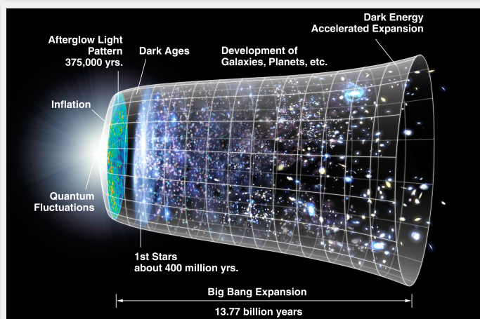
Fig 4. The timeline of the universe's expansion is illustrated with circular sections representing space, including hypothetical, unobservable regions, at each point in time. At the very beginning is the big bang epoch, followed by a rapid expansion during the inflationary epoch, while at the center, the expansion begins to accelerate.
